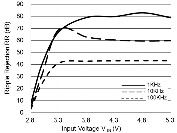
Ripple Rejection vs. Input Bias Voltage AP7340-28 I_{OUT}=30mA
