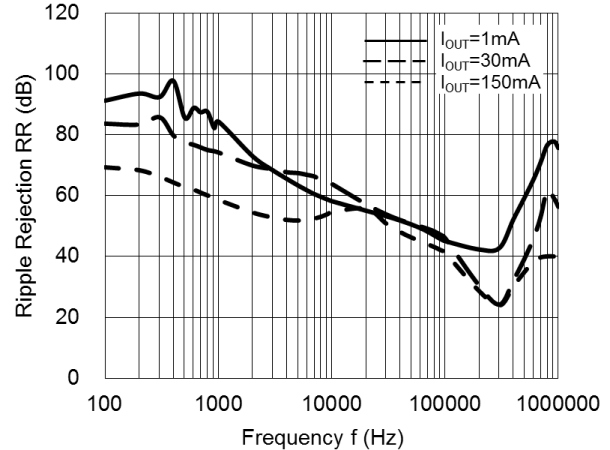
Ripple Rejection vs. Frequency AP7340-33
